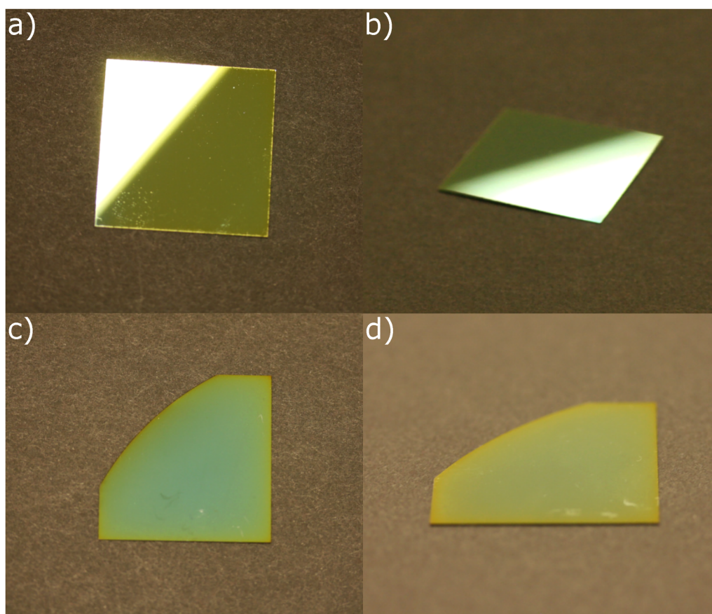
FIG. 4. Photographs of the polished (a) and (b) and textured (c) and (d) sample, taken under office lighting at 15^\circ [(a) and (c)] and 60^\circ [(b) and (d)]. The same black paper is used as background for all samples, but seems to have a different color in some photographs due to variations in the camera exposure time. The polished substrates are 30 \times 30 mm, and the textured ones have a radius of 30 mm.
