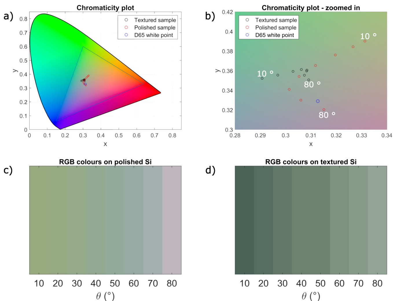
FIG. 3. Chromaticity diagram of the polished and textured samples at angles of incidence 10^\circ to 80^\circ (a), with additional zoom around the relevant area (b), together with color patches of the polished (c) and textured (d) samples at angles of incidence 10^\circ to 80^\circ .
