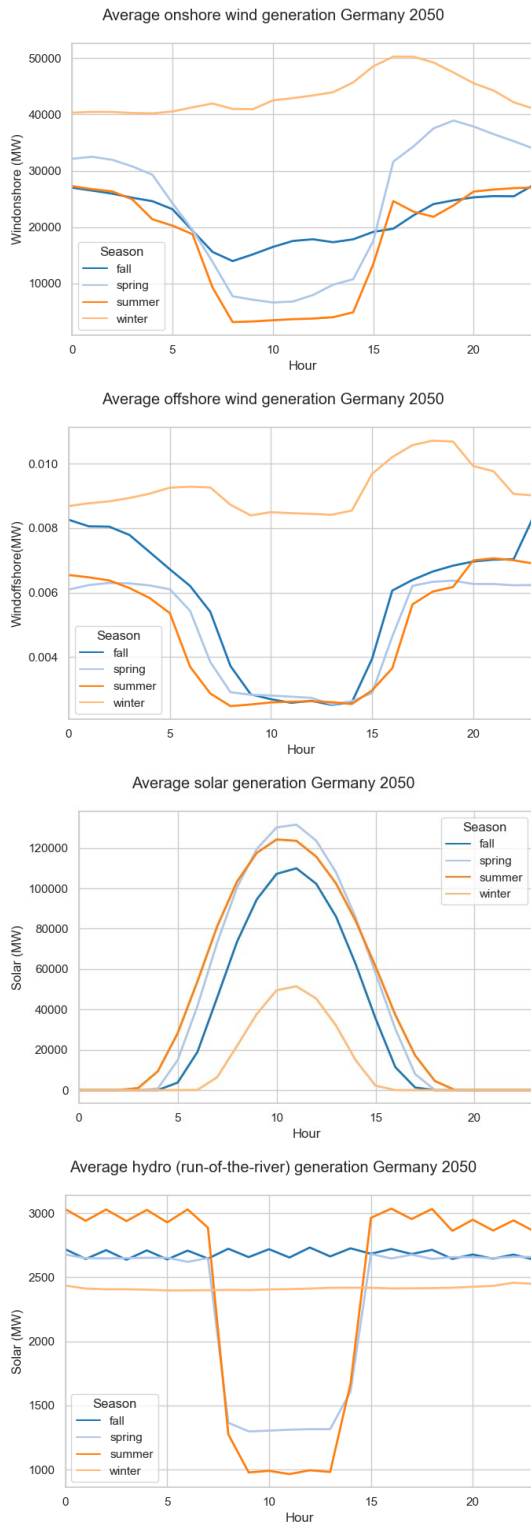
Figure 87. Average power production for non-dispatchable technologies in Germany 2050.
