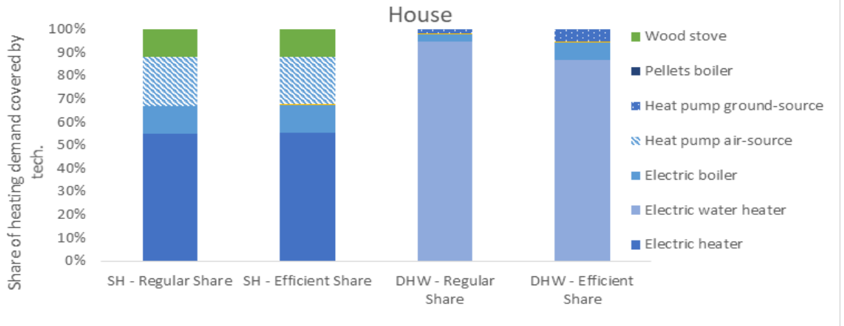
Figure 35. Share of energy demand for space heating and domestic hot water heating being covered by different heating technologies in single family houses in 2020.
