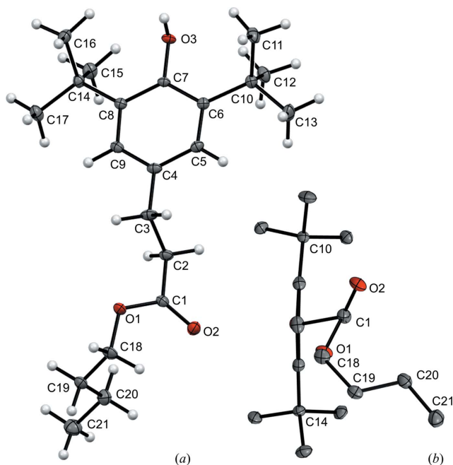
Figure 2 (a) The molecular structure of (I) at 100 K. Thermal displacement ellipsoids are shown at the 50% probability level. (b) Rotated view, H atoms excluded.
