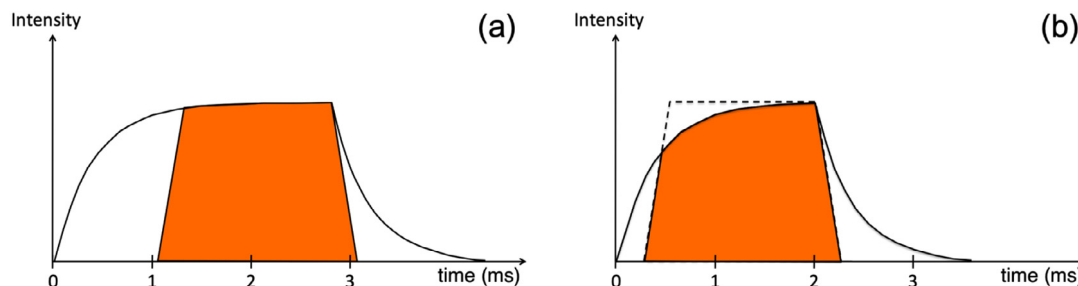
Fig. 2. Pulse-shaping chopper with a 1.5 ms opening, using a 2.86 ms (a) and a 2.00 ms source pulse (b).
