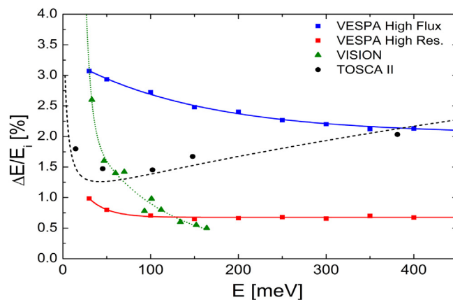
Fig. 38. VESPA relative resolution as a function of the energy transfer: blue squares represent the ‘high flux’ mode, while red squares the ‘high resolution’ mode. VISION and TOSCA-II estimated performances [112,114] are reported as green triangles and black circles, respectively. Lines are only a guide for the eye.
