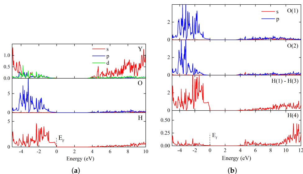
Figure 7. Electron structure of Y_2H_3O(OH) in terms of density of states (DOS): The Fermi level is shifted to a zero value. The highest valence band state and the lowest conduction band state at the Brillouin zone center determine the fundamental band-gap width of 3.4 eV. (a) Element-projected partial density of states. (b) Site-projected partial density of states. H(1)–H(3) positions relate to the hydride anion; H(4) describes the proton in the hydroxide anion.
