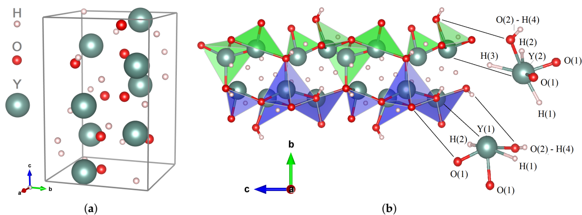
Figure 2. Predicted crystal structure of Y_2H_3O(OH) : The structural parameters are given in Table 1. (a) A schematic view of the unit cell along the tetragonal c axis. (b) A characteristic pattern of polyhedral chains viewed along a axis.
