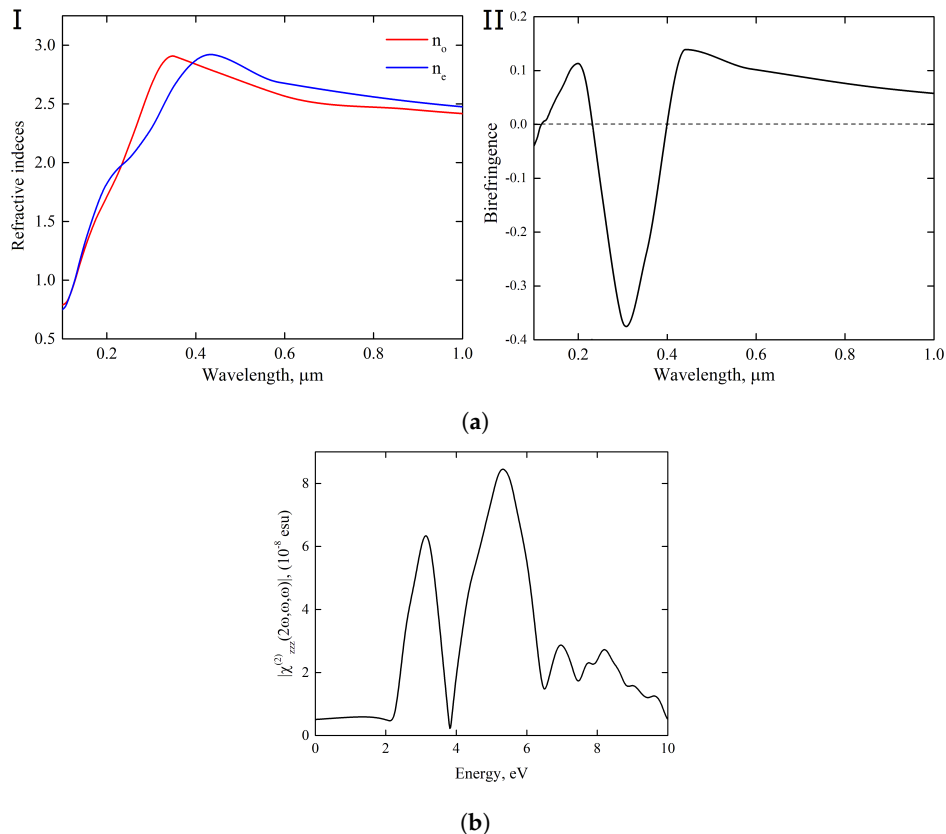
Figure 8. Optical responses: (a) The phenomena of anomalous dispersion of refractive indices (I) and of anomalous birefringence ( \Delta n = n_e - n_o ) (II) in uniaxial \text{Y}_2\text{H}_3\text{O}(\text{OH}) . The optic axis is fixed in the z direction. In subsection (II), crossing of the dashed line with the birefringence curve indicates \lambda = 117 , 231, and 401 nm as isotropic points in the given spectral region. (b) Prediction of the second-harmonic generation (SHG) spectrum of \text{Y}_2\text{H}_3\text{O}(\text{OH}) represented in terms of the spectral behavior of the absolute value of the second-order susceptibility tensor component \chi_{zzz}(2\omega, \omega, \omega) .
