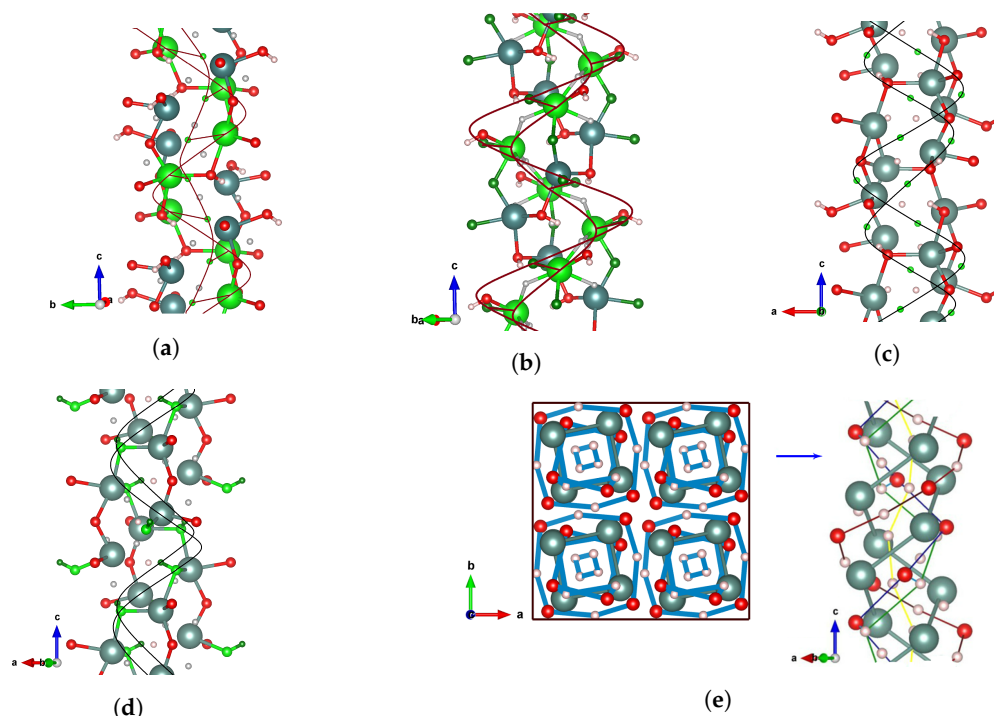
Figure 6. Scheme of a chiral packing composed of the circular helices with pitch of 9.264 \text{ \AA} : The color codes of atoms are the same as in Figure 2. The helical structures were parametrized in terms of functions x(t) = a \cos(t) , y(t) = a \sin(t) , and z(t) = bt , where a is the radius and the ratio b/a represents the slope. (a) Helical chains formed by Y(1) and H(3). Y(1): a = 2.17 \text{ \AA} , b/a = 0.68 ; H(3): a = 0.75 \text{ \AA} , b/a = 1.97 . (b) Helical chains formed by Y(2) and O(1). Y(2): a = 2.17 \text{ \AA} , b/a = 0.68 ; O(1): a = 3.28 \text{ \AA} , b/a = 0.45 . (c) Helical chains formed by H(1) and H(2). H(1): a = 2.27 \text{ \AA} , b/a = 0.65 ; H(2): a = 2.84 \text{ \AA} , b/a = 0.52 . (d) Helical chains formed by O(2) and H(4). O(2): a = 2.17 \text{ \AA} , b/a = 0.68 ; H(4): a = 1.94 \text{ \AA} , b/a = 0.76 . (e) Packing motif of the helical structure in the unit cell. A column composed of six joined helical chains represents the building block of the chiral framework of Y_2H_3O(OH) . The internal tunnel is filled by the single H(3) helical chain.
