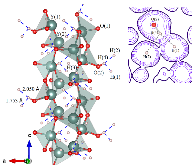
Figure 5. Chains of yttrium polyhedral units linked by dihydrogen bonds in the Y_2H_3O(OH) crystal structure: The blue dashed lines denote the relevant H \cdots H contacts. The color codes of atoms are the same as in Figure 2. At the right, 2D contour plot of the valence electron density, calculated at ELF = 0.8475 , presents O(2)-H(4) \cdots H(1) and O(2)-H(4) \cdots H(2) dihydrogen bonding connections. According to the AIM protocol for charge densities, the minimum distances to a zero flux surface are located at distances of about 0.809, 0.816, and 0.159 Å for the H(1), H(2), and H(4) sites, respectively.
