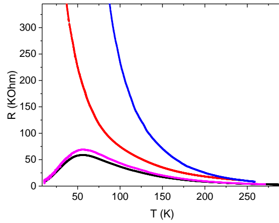
Figure 1: Temperature dependence of resistance in different areas of GdOH films (shown in different color) deposited on borosilicate glass. A decrease in resistance at temperature below 60 K has been observed in some areas.
