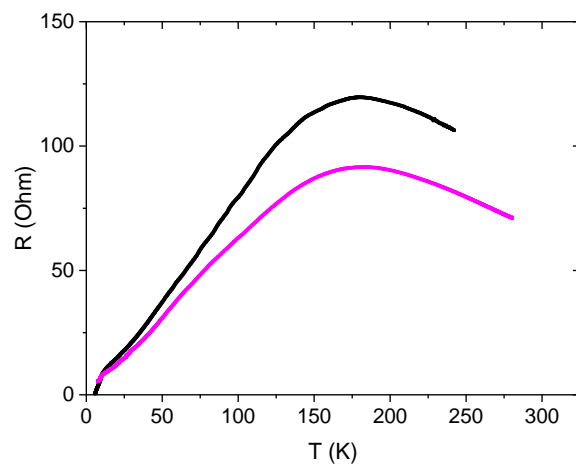
Figure 2: Temperature dependence of resistance for different areas of GdOH films deposited on SrTiO 3 single-crystalline substrate shown in different color. A decrease in resistance has been observed at temperature below 180 K.
