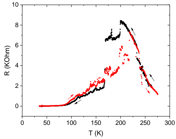
Figure 3: Temperature dependence of resistance for GdOH film deposited on Si single-crystalline substrate. In spite of hysteresis and irreproducible jumps coming from the contacts, an apparent zero resistance is observed at temperatures below 40 K.
