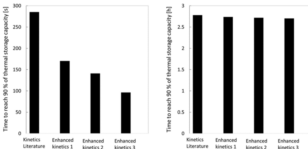
Fig. 4 – The impact on the system performance due to enhancement of reaction kinetics for 0.2 g (left) and 30 kg (right) of metal powder. Increasing the rate of reaction has a significantly greater impact on the smaller system (a) than on the larger system (b).
