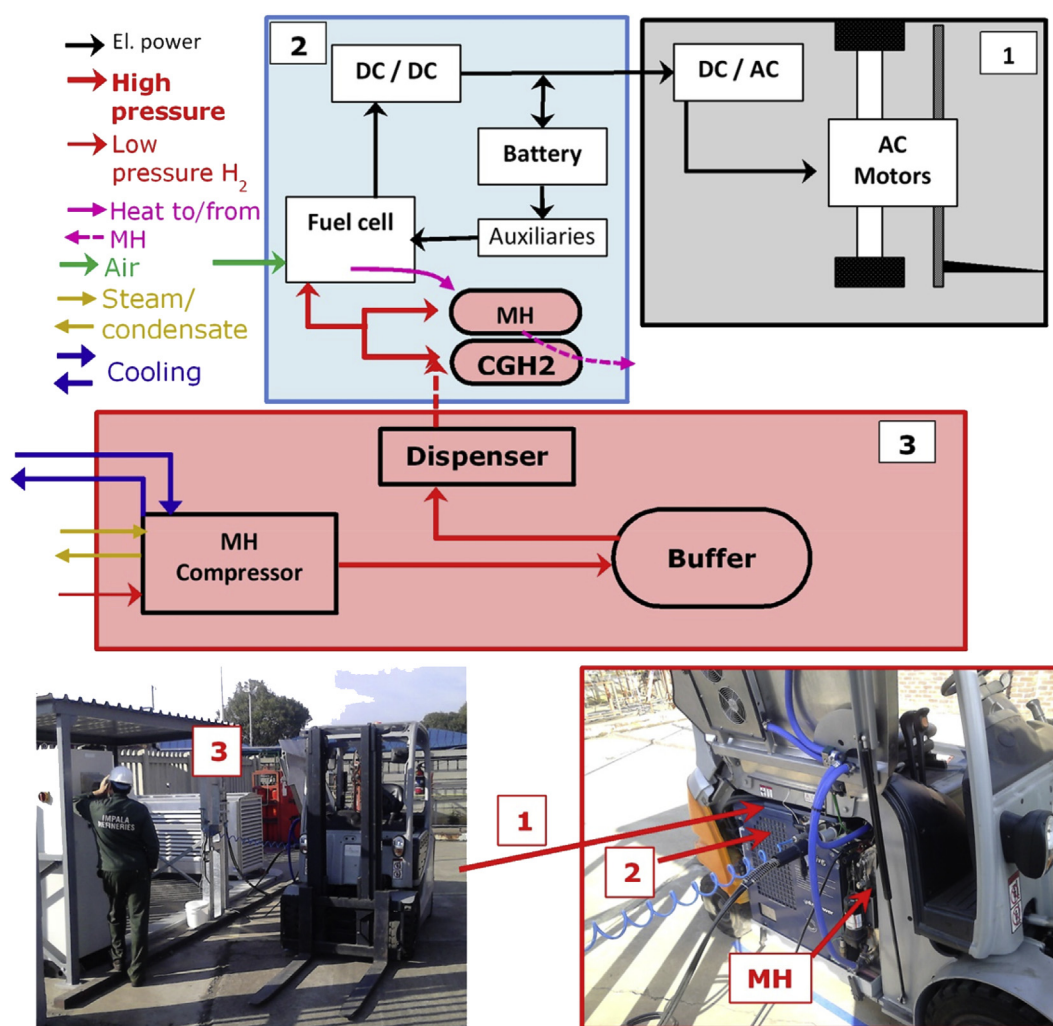
Fig. 10 – Top: general system concept, bottom: prototypes of FC/MH forklift and MH based H 2 refueling station (Implats refineries, South Africa). 1 –forklift, 2 – fuel cell power module with integrated H 2 storage, 3 – refueling system. Technical characteristics: full-load (VDI-60) operation time 3.1 h 2 , average power 10 kW. Mass of the MH system 250 kg 3 . Useable H 2 capacity 1.83 kg. Hydrogen charging pressure 185 bar. Charging time 6–15 min.
