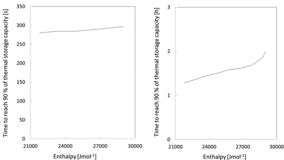
Fig. 3 – The impact on system performance due to increases reaction enthalpy for 0.2 g (left) and 30 kg (right) of metal powder. Increasing reaction enthalpy has a greater degree of impact on the larger system (b) than on the smaller system (a).
