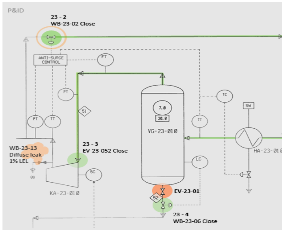
Figure 8: Process and instrumentation diagram
